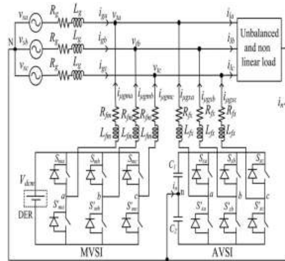
Fig.4. Topology of DVSI scheme
